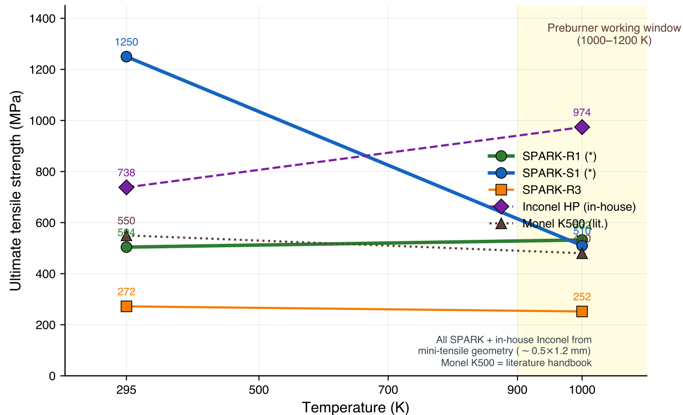
Strength retention at temperature · SPARK candidates vs benchmarks
