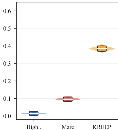
I_{\text{KREEP}} (trace-element potential)
