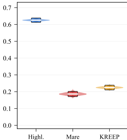
I_{\text{AlCa}} (highlands potential)
