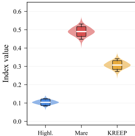
I_{\text{FeTi}} (mare potential)
