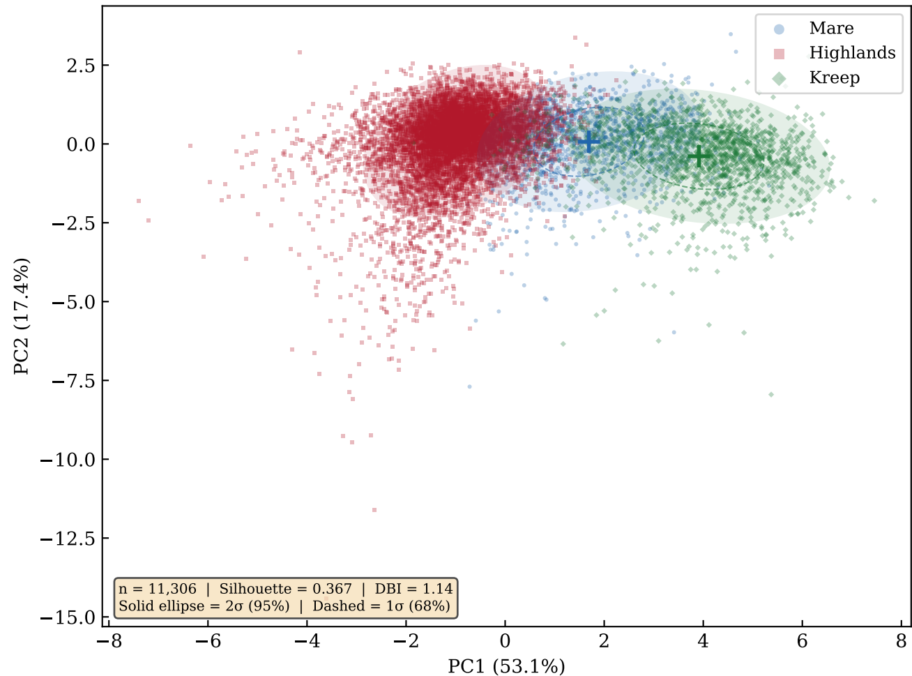
PCA: Terrane Separation in Geochemical Space (2-deg LP-GRS)
