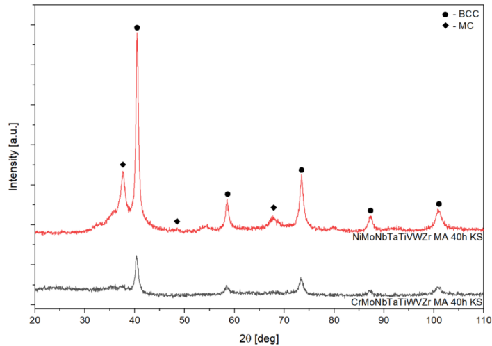
(b) 8-element MA powders: BCC matrix
