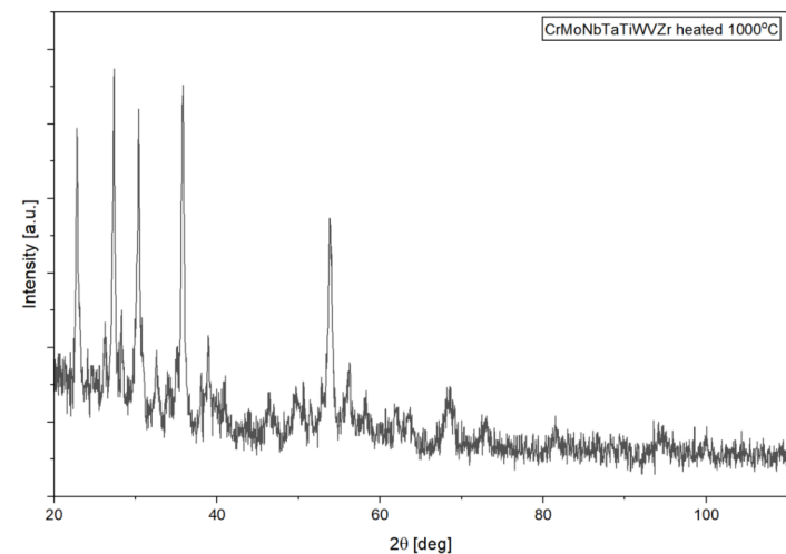
(c) 8-element compact at 1000 °C: phase decomposition
