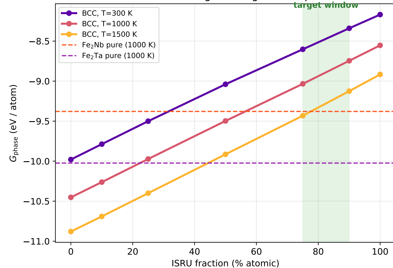
Phase free energies along dilution path
