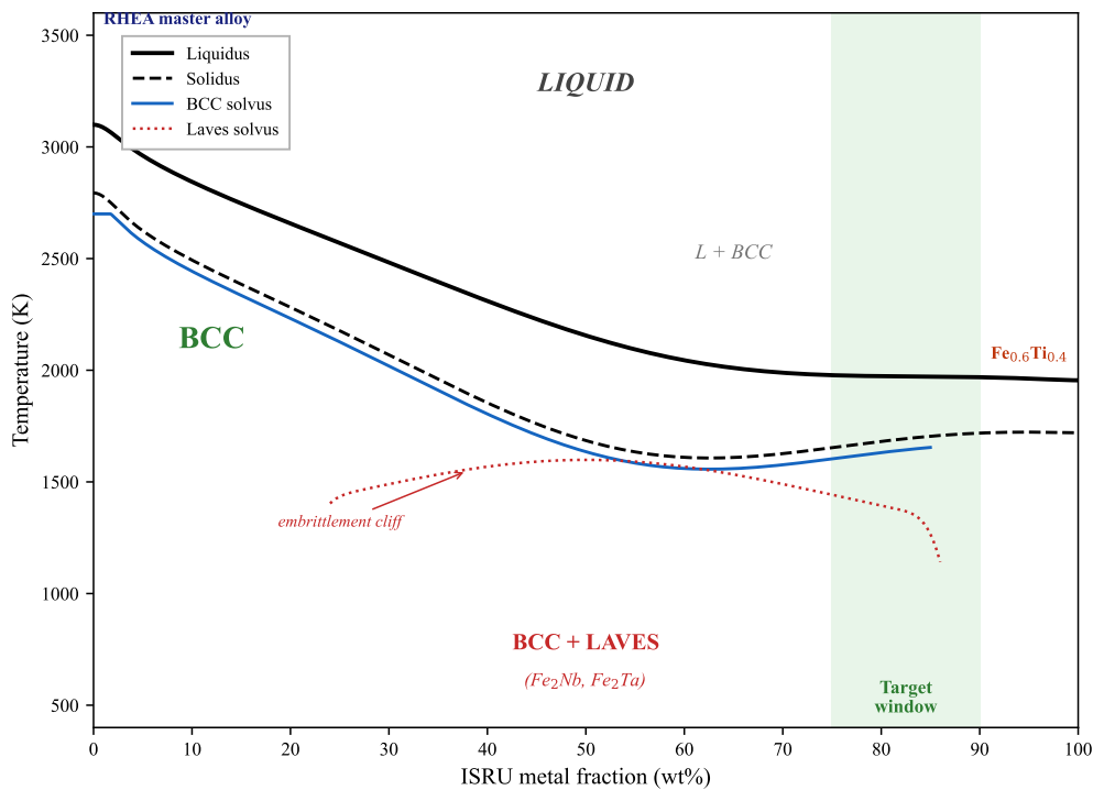
Figure 12: Schematic pseudo-binary phase diagram for the dilution trajectory from a concentrated RHEA master alloy (left) to ISRU-derived Fe–Ti bulk metal (right). Phase boundaries are constructed from the Fe–Ti binary (COST507, well-characterised) with refractory interaction effects informed by published HEA literature [7, 9]. The green band marks the target dilution window (75–90 wt% ISRU), where the hybrid alloy is expected to retain a single-phase BCC structure with solid-solution strengthening from dissolved refractory elements. The Laves-phase field ( \text{Fe}_2\text{Nb} , \text{Fe}_2\text{Ta} ) at intermediate compositions represents the embrittlement cliff that must be avoided. Note: this diagram is illustrative; quantitative phase boundaries require TCHEA-grade CALPHAD calculations for specific RHEA+Fe–Ti pseudo-binaries.
