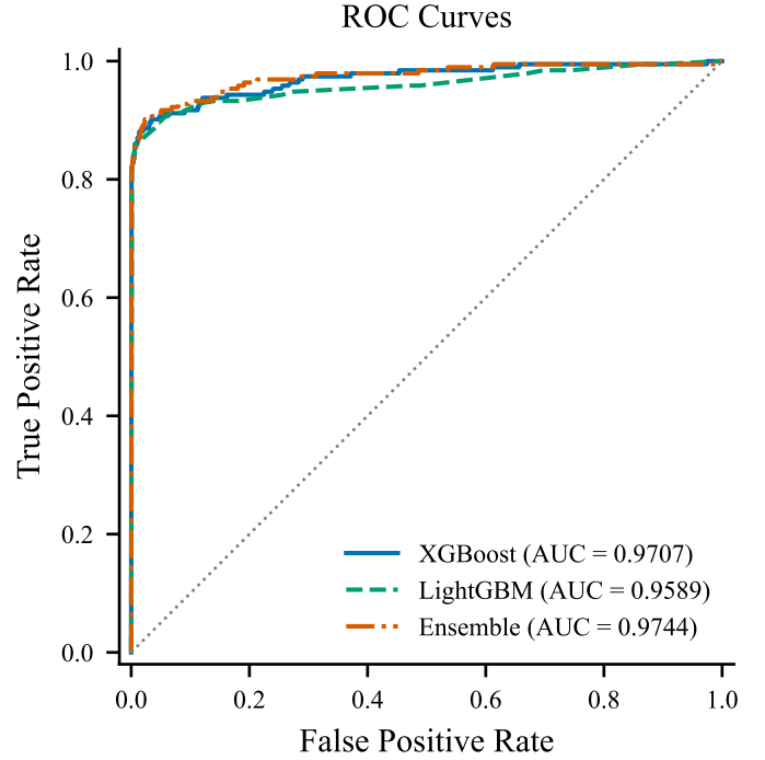
Fig. 3: ROC curves for XGBoost, LightGBM, and the ensemble on the held-out test set.
