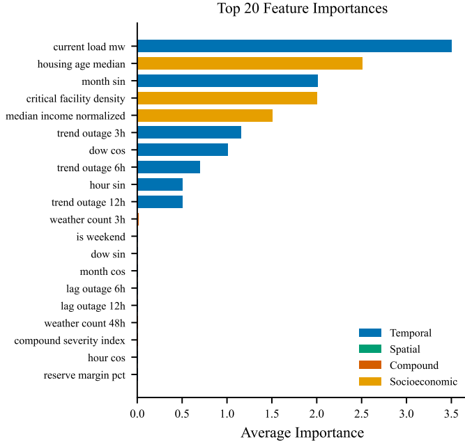
Fig. 2: Top 20 features by average importance across XGBoost and LightGBM, color-coded by group: temporal (blue), spatial (green), compound (red), socioeconomic (orange).
