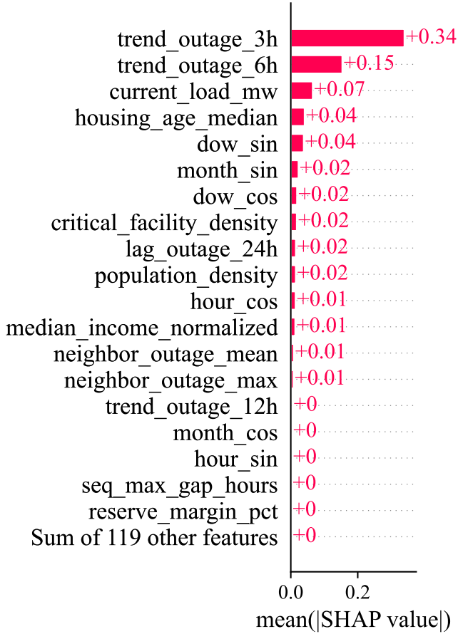
Fig. 3: SHAP mean absolute values for the top 20 features, providing model-agnostic feature importance.
