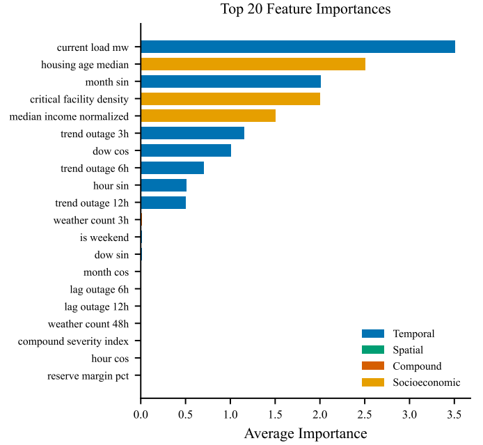
Fig. 2: Top 20 features by average importance across XGBoost and LightGBM, color-coded by group: temporal (blue), spatial (green), compound (red), socioeconomic (orange).
