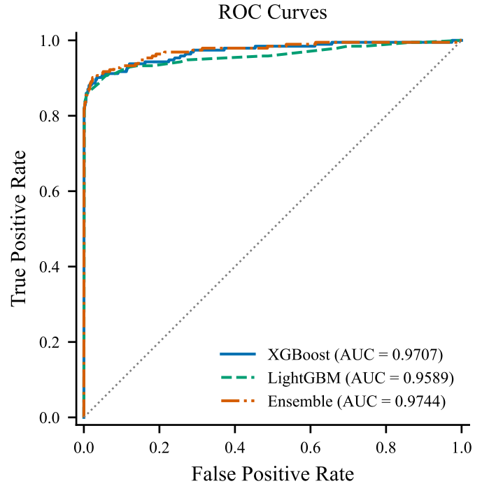
Fig. 4: ROC curves for XGBoost, LightGBM, and the ensemble on the held-out test set.
