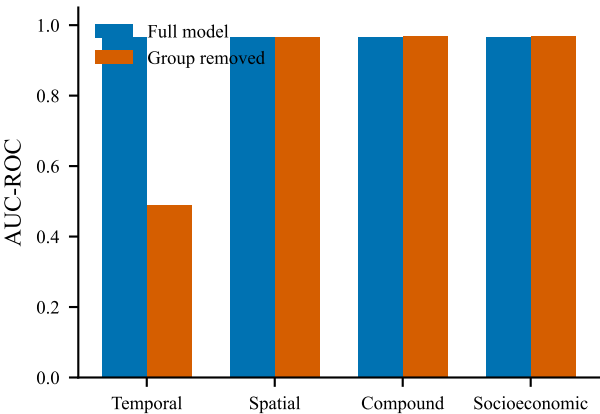
Ablation Study: AUC-ROC by Feature Group
