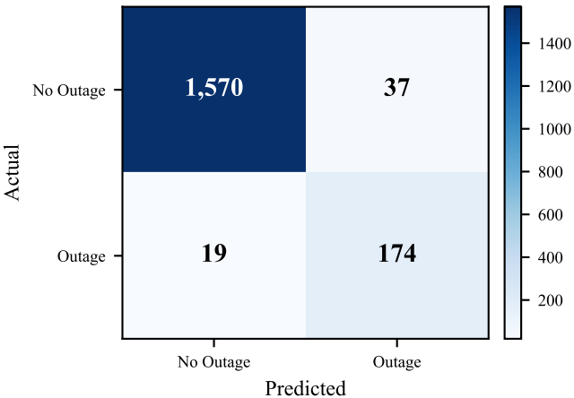
Confusion Matrix (threshold = 0.297)
