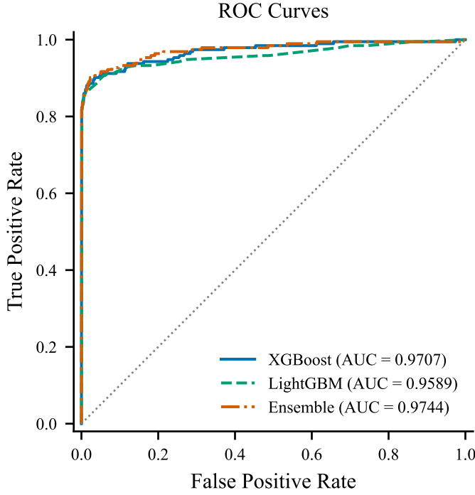
Fig. 4: ROC curves for XGBoost, LightGBM, and the ensemble on the held-out test set.
