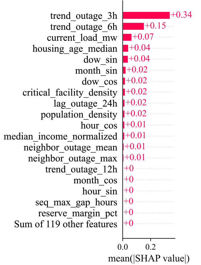
Fig. 3: SHAP mean absolute values for the top 20 features, providing model-agnostic feature importance.
