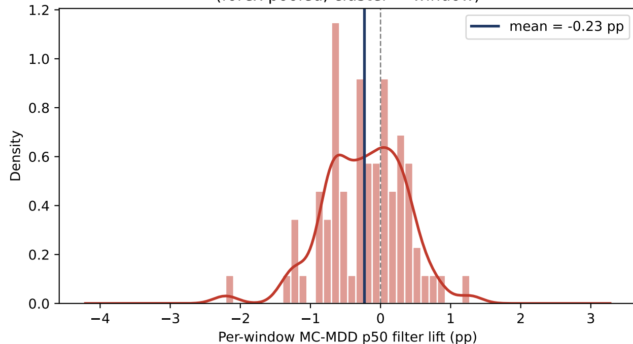
(A) Window-level MC-MDD filter lift distribution (forex pooled, cluster = window)
