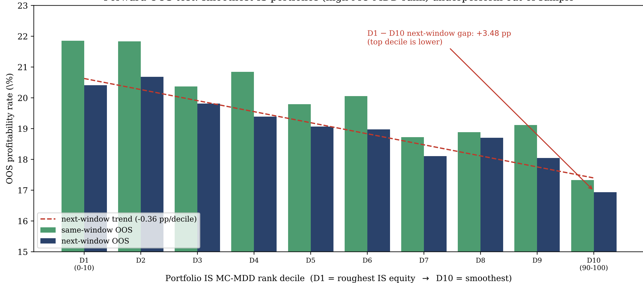
Forward-OOS test: smoothest-IS portfolios (high MC-MDD rank) underperform out-of-sample
