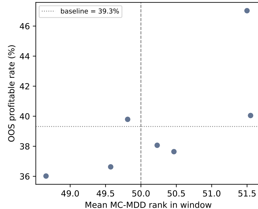
SOL: per-window MC-MDD rank vs OOS profitability (7 windows)
