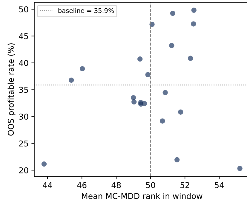
DOGE: per-window MC-MDD rank vs OOS profitability (21 windows)
