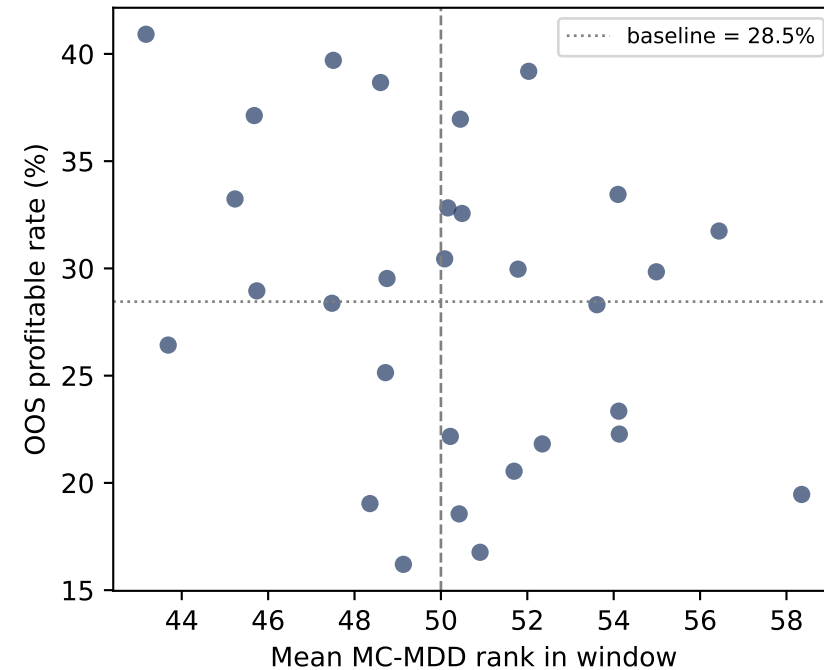
BNB: per-window MC-MDD rank vs OOS profitability (30 windows)
