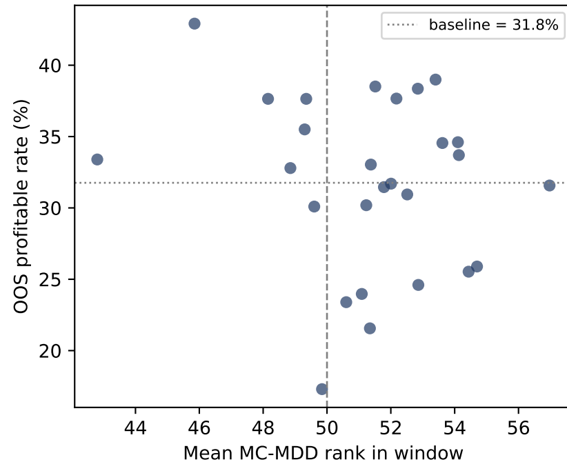
BTC: per-window MC-MDD rank vs OOS profitability (27 windows)
