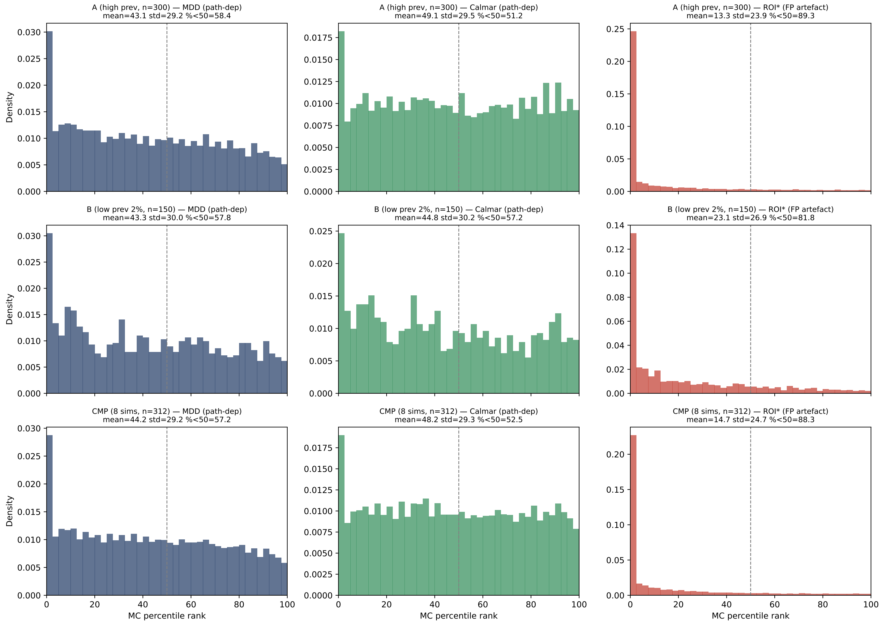
Fig 5: synthetic-pipeline MC rank distributions — MDD/Calmar (informative) vs ROI* (FP artefact)
