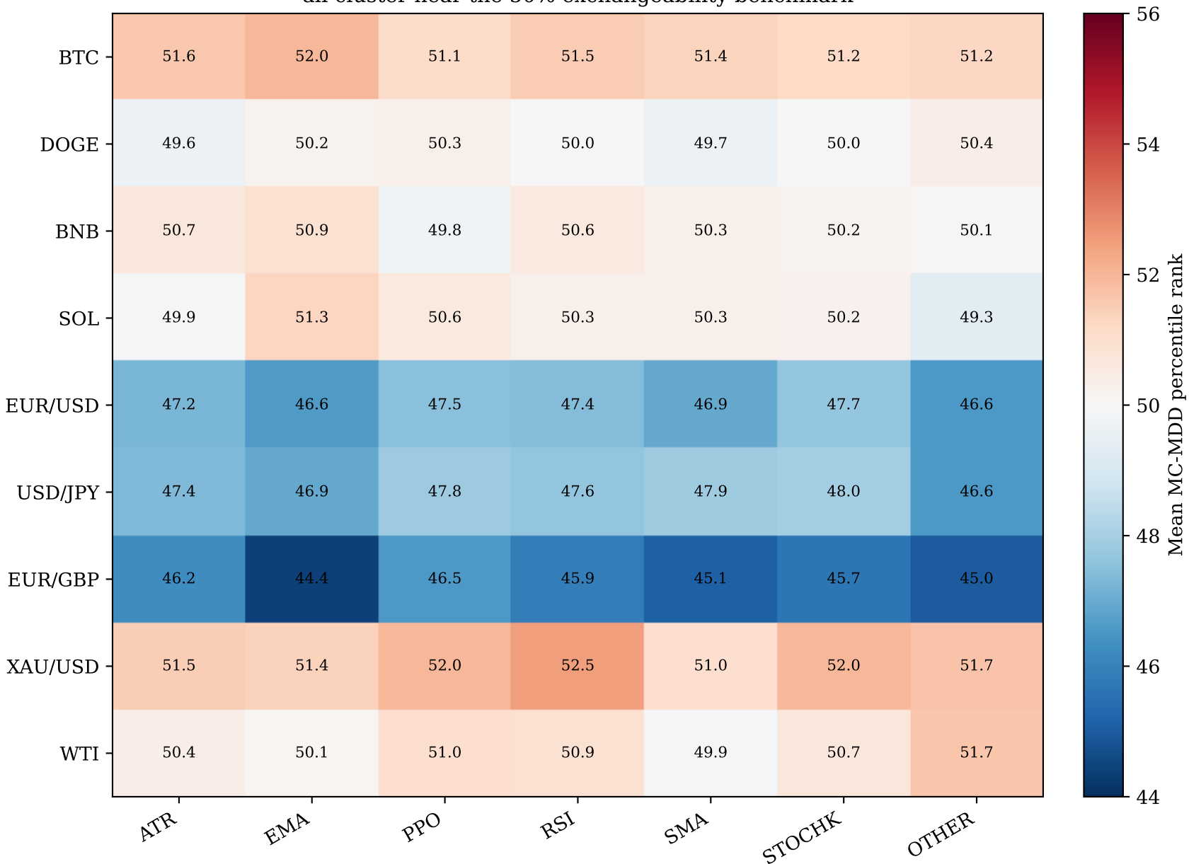
MC-MDD rank means by asset \times indicator family (63 cells): all cluster near the 50% exchangeability benchmark
