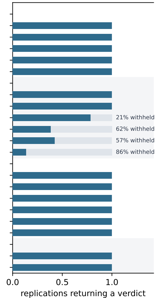
Where the abstention rule fires
