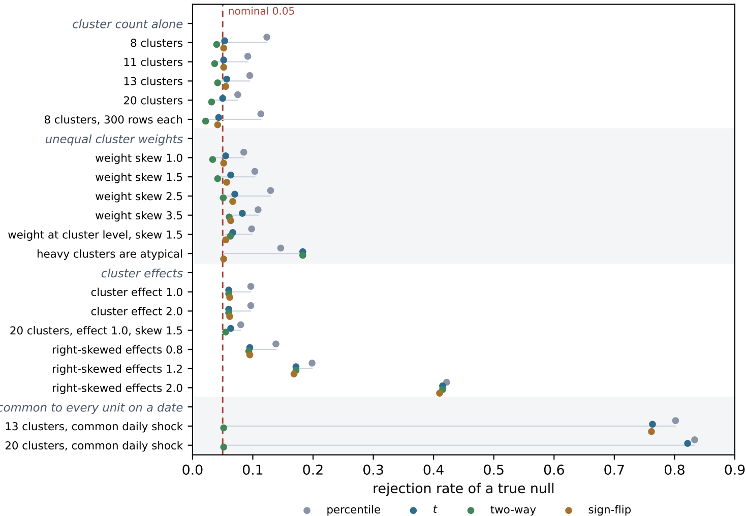
Size of four interval methods
