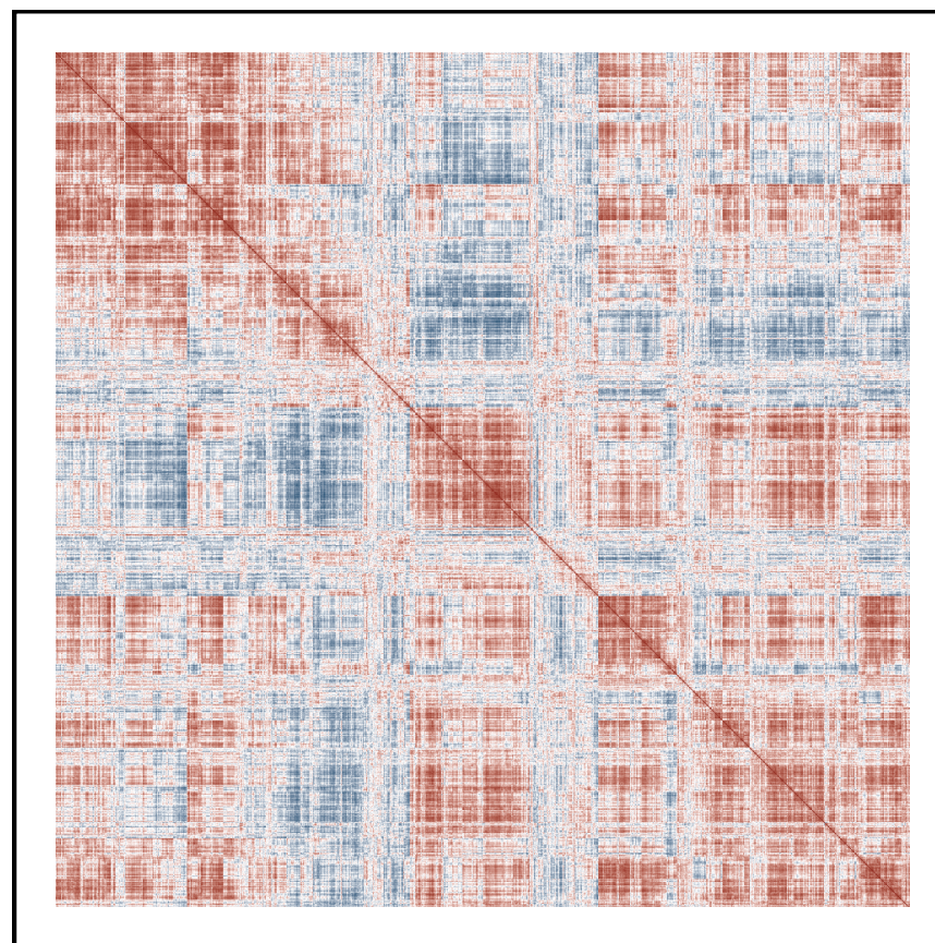
CCl 4 protein data
