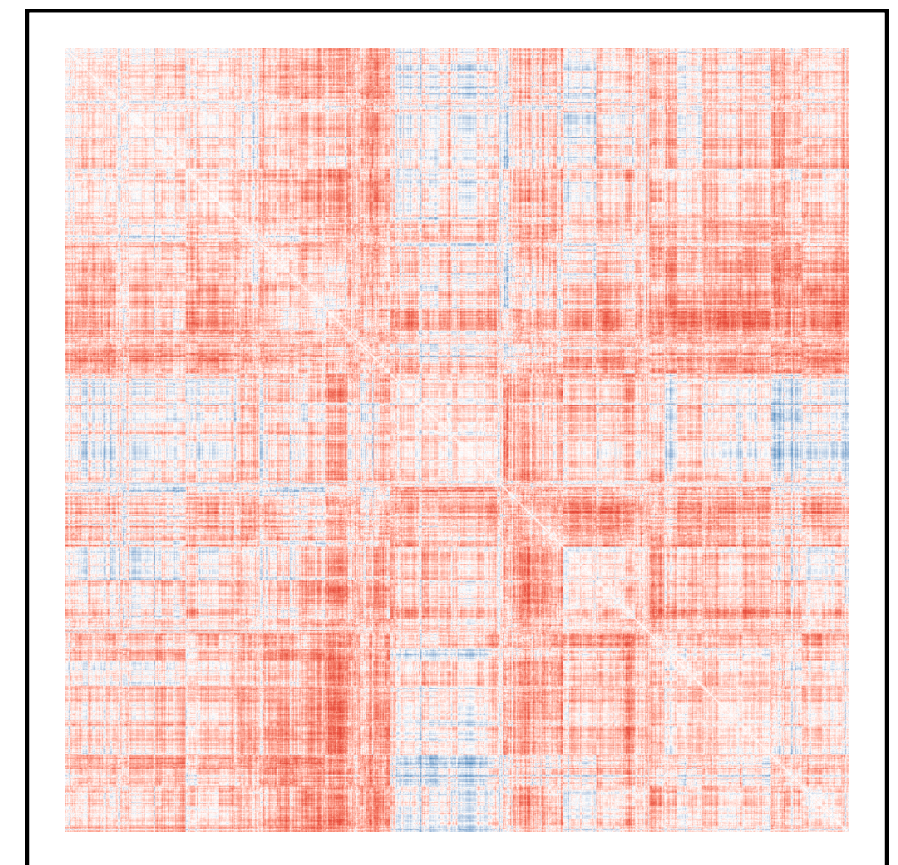
Difference of BDL on CCl 4 data
