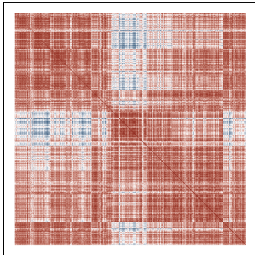
BDL protein data
