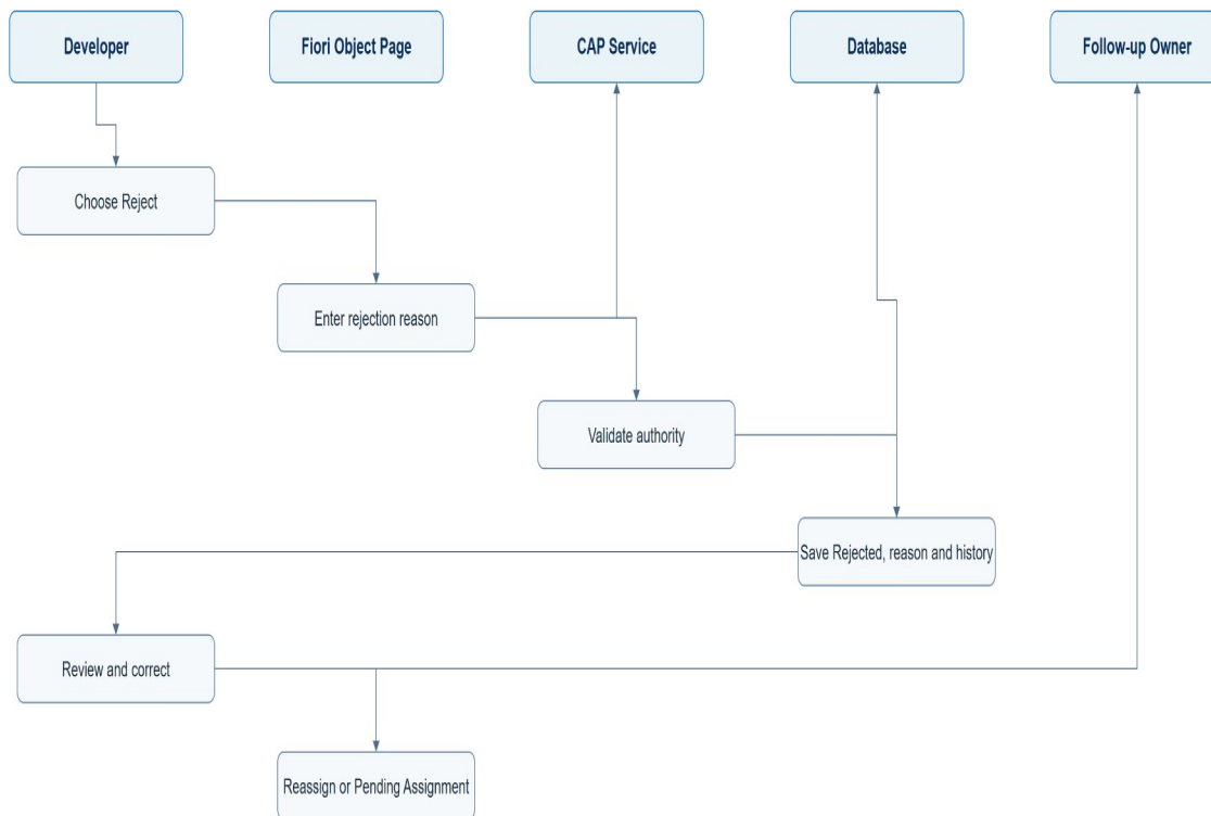
Figure 15. Rejected Follow-up Flow. IDTS Diagram Pack; editable master is maintained as a draw.io file with the project artifacts.
