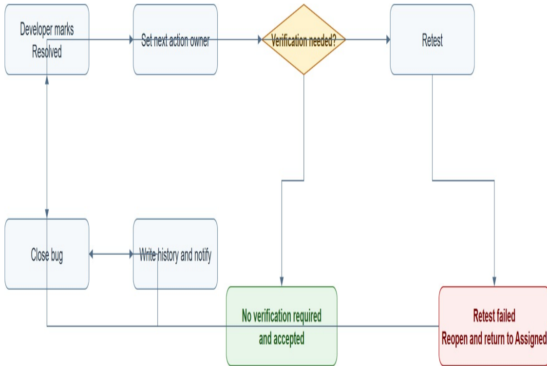
Figure 20. Resolve, Retest, Close, and Reopen Flow. IDTS Diagram Pack; editable master is maintained as a draw.io file with the project artifacts.
