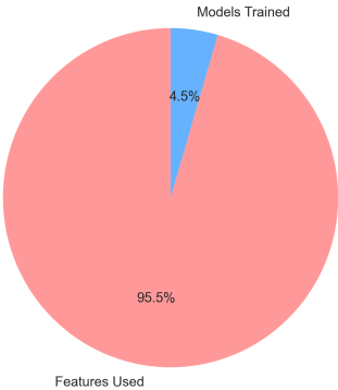
Training Summary
