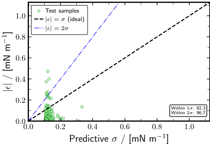
Error vs Uncertainty Calibration
