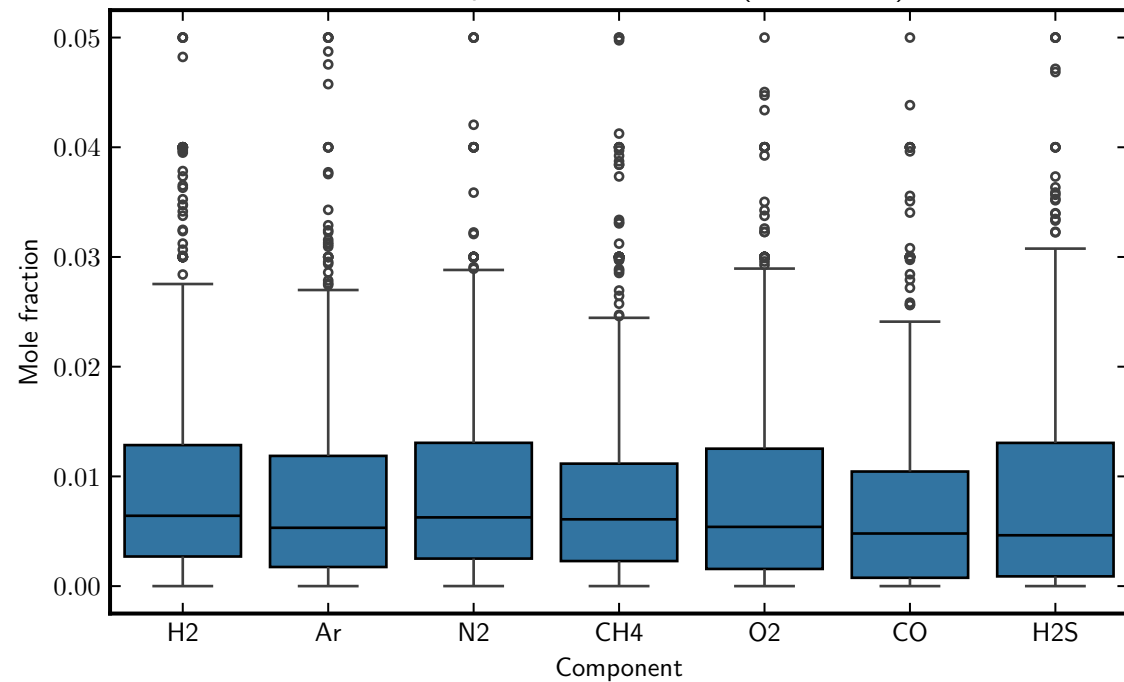
Minor component distributions (M = 1,000)
