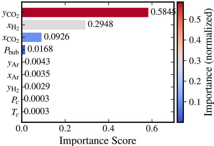
Feature Importance (Random Forest)
