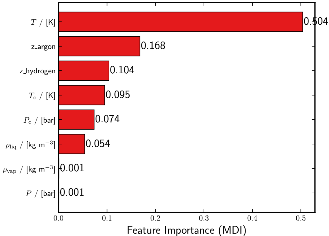
Random Forest — Feature Importances
