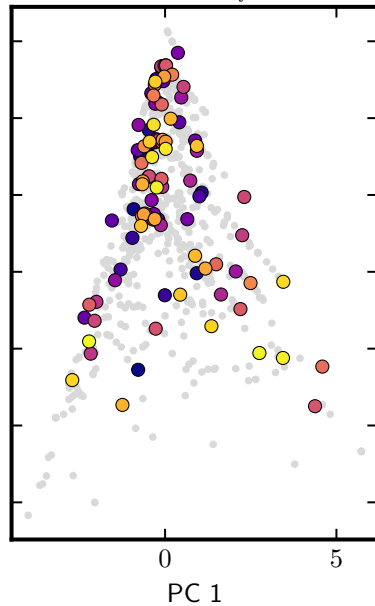
T = 0.1 \sigma_f^{2*}
