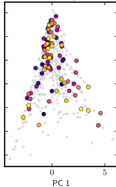
T = 10 \sigma_f^{2*}
