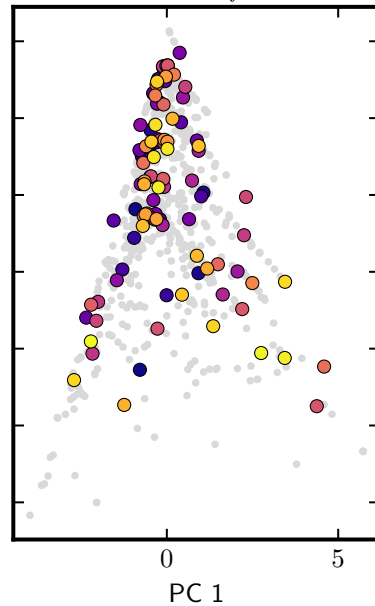
T = 1 \sigma_f^{2*}
