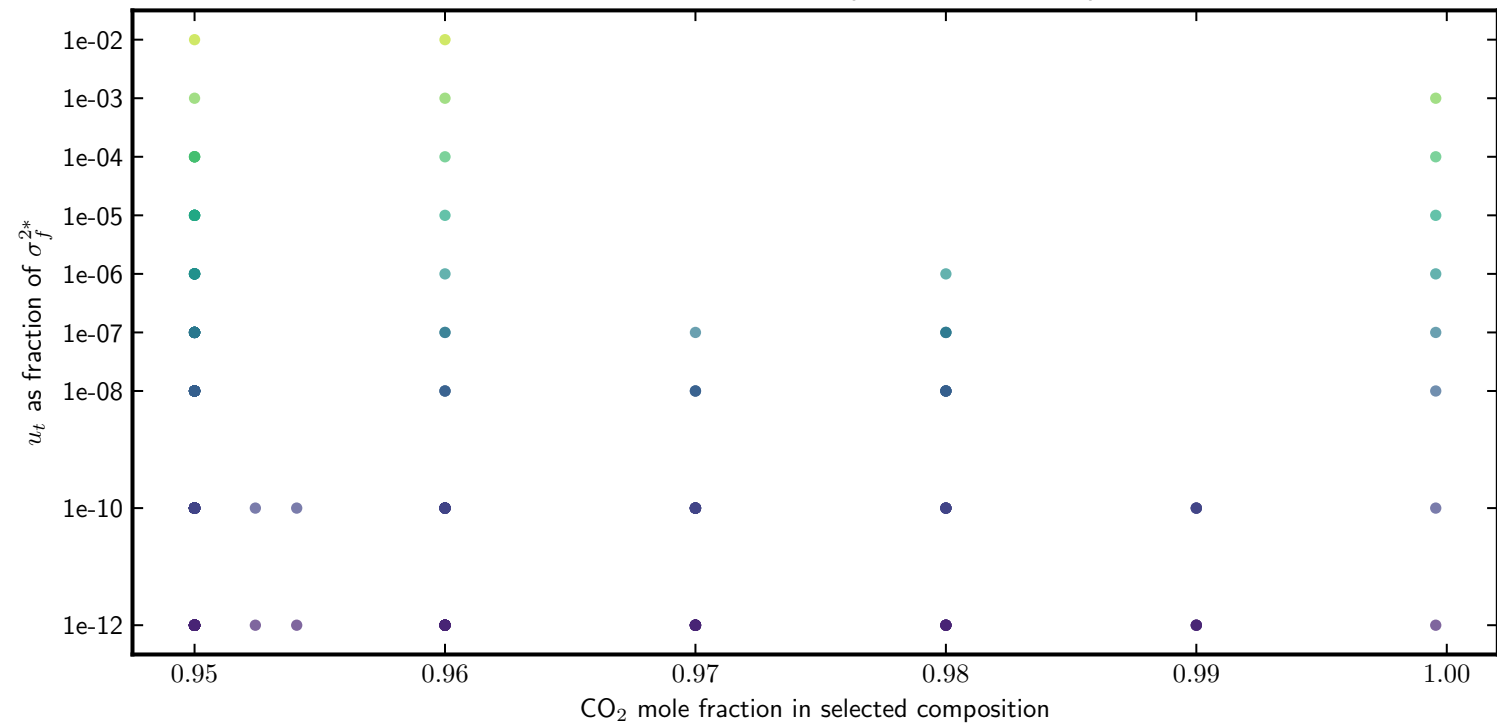
Distribution of selected compositions in CO 2 space
