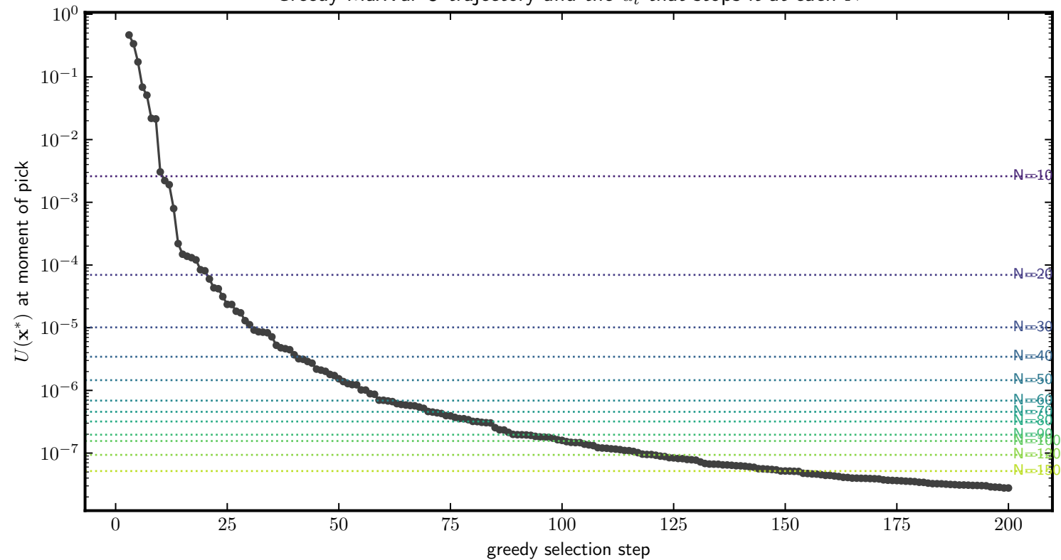
Greedy MaxVar U trajectory and the u_t that stops it at each N
