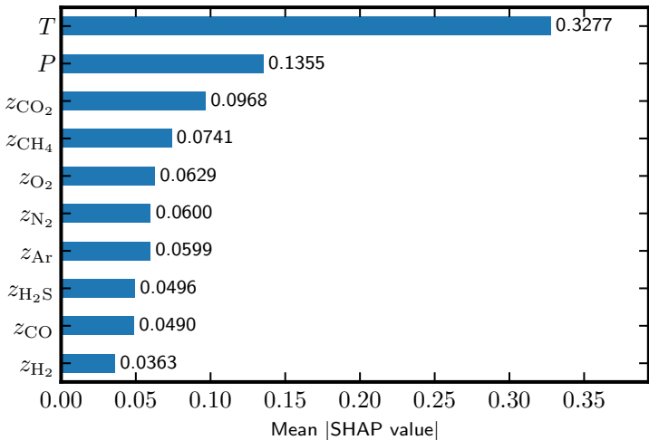
SVR (RBF) Feature Importance — \ell_{\text{if}}
