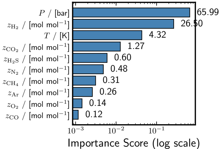
Feature Importance (Log Scale)
