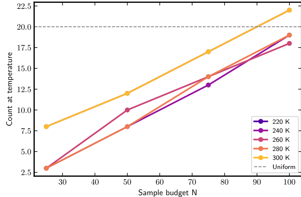
Temperature distribution in AL selection
