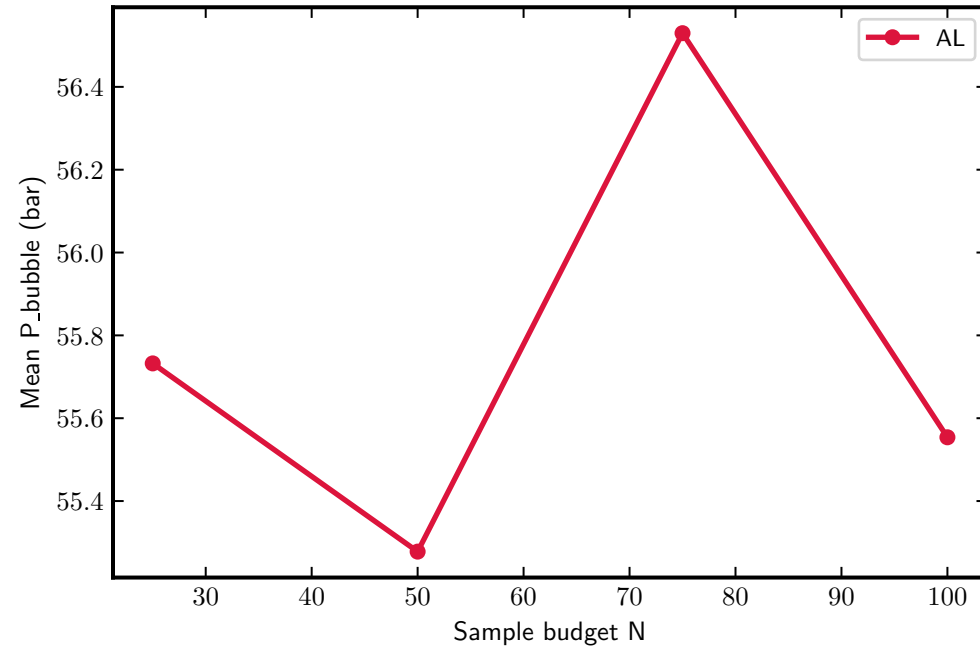
Mean bubble-point pressure vs N (over 5 temperatures)
