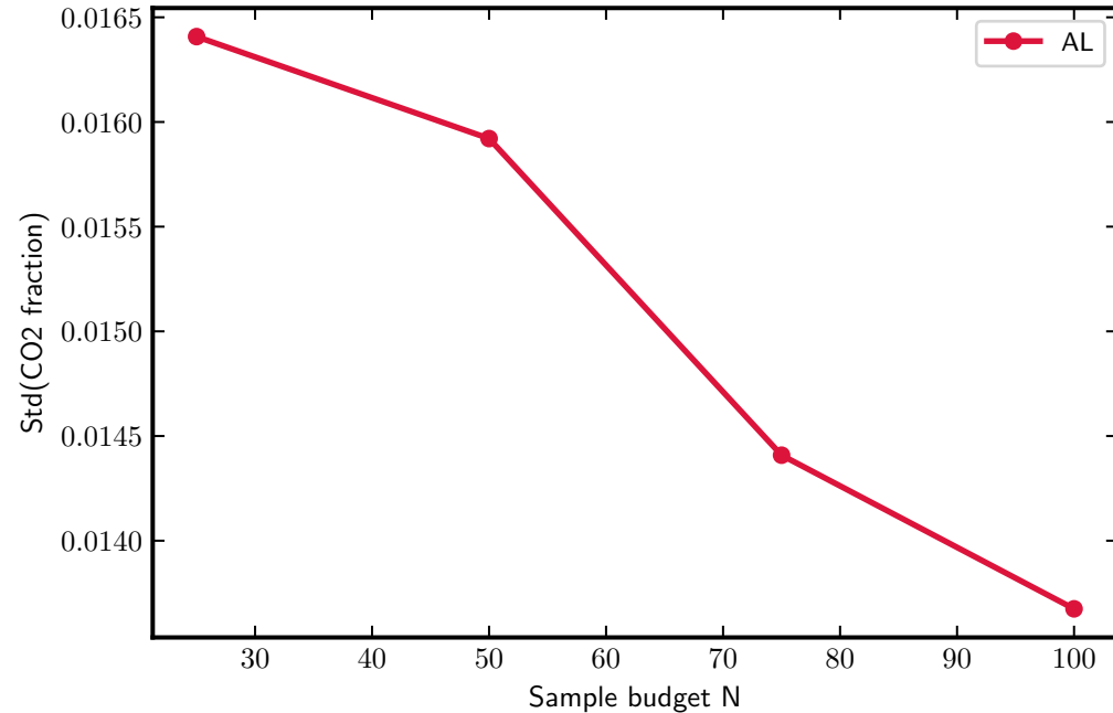
CO 2 fraction diversity vs N
