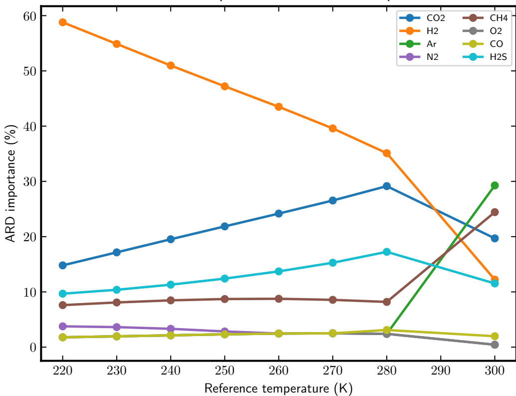
ARD feature importance vs reference temperature
