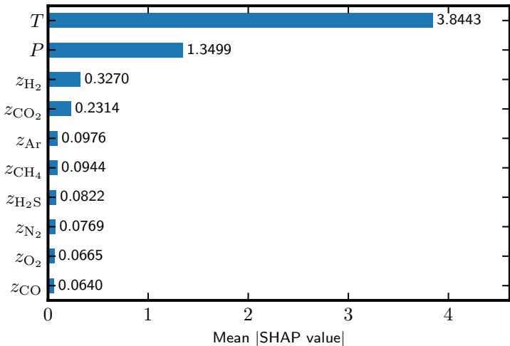
SVR (RBF) Feature Importance — \gamma
