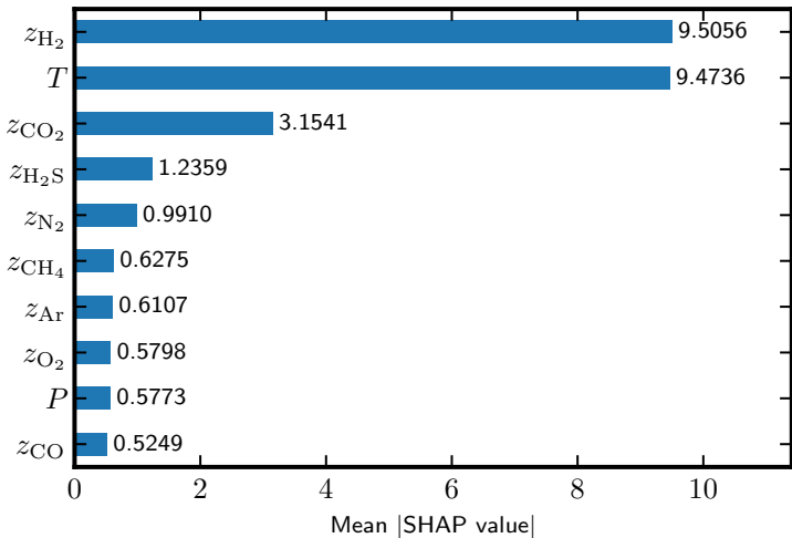
SVR (RBF) Feature Importance — P_{\text{bubble}}
