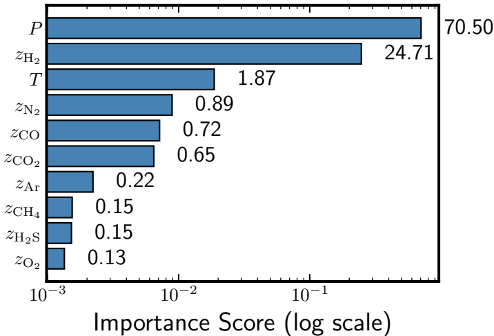
Feature Importance for P_{\text{bubble}} (Log Scale)
