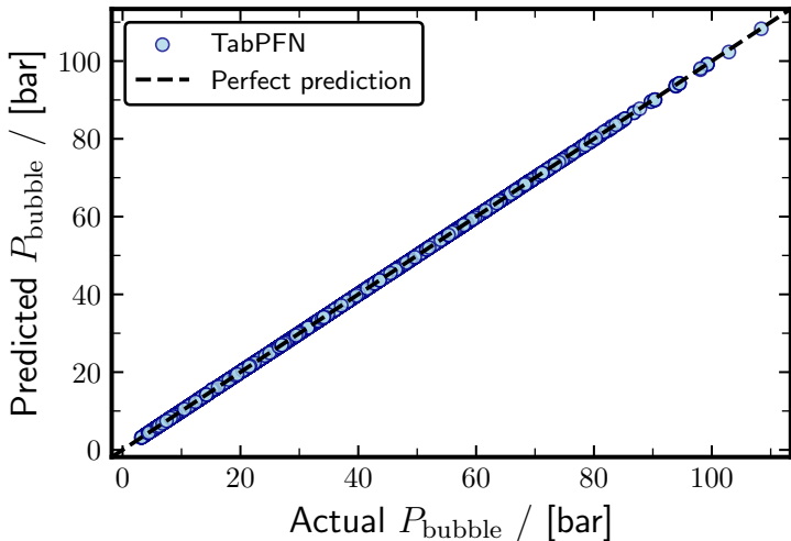
TabPFN Parity Plot (Test Set)
