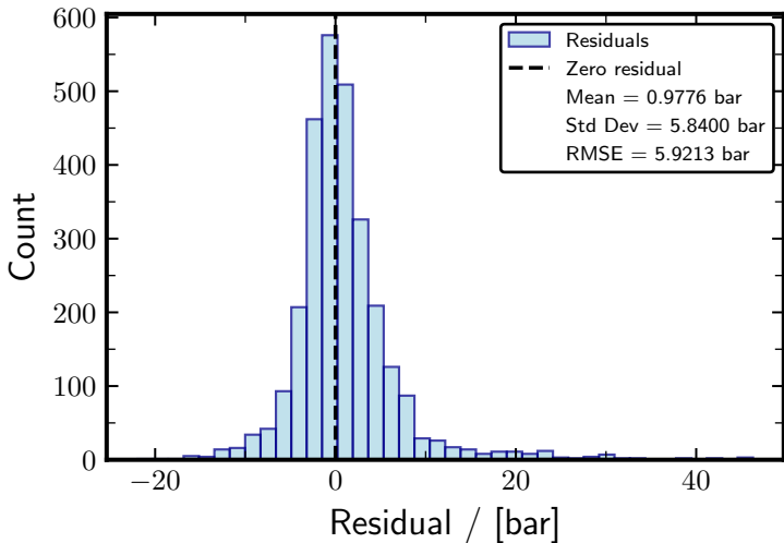
Residual Distribution
