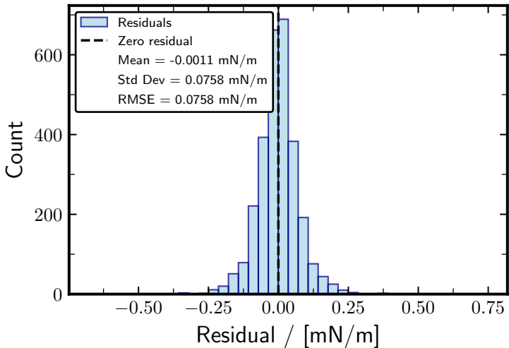
Residual Distribution
