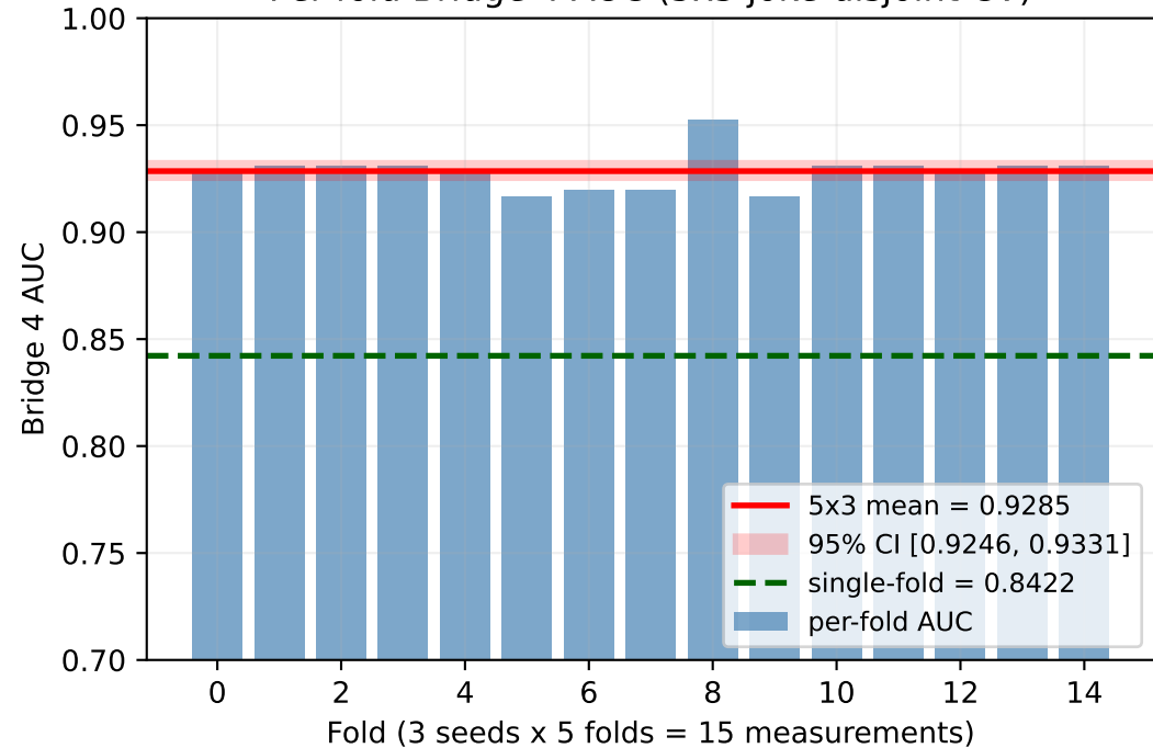
Per-fold Bridge 4 AUC (5x3 joke-disjoint CV)
