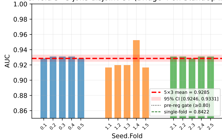
Per-fold 5×3 joke-disjoint CV (Bridge 4 on StandUp4AI)
