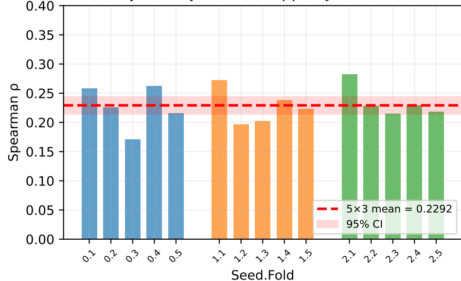
Per-fold 5×3 joke-disjoint CV (SeppeV Jester, RoBERTa-base)
