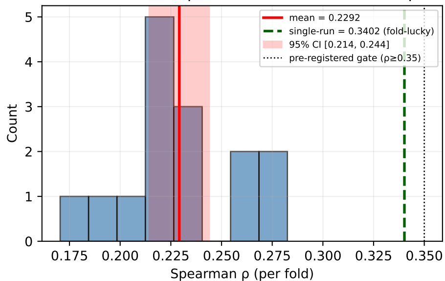
Distribution of 15 \rho measurements + bootstrap CI
