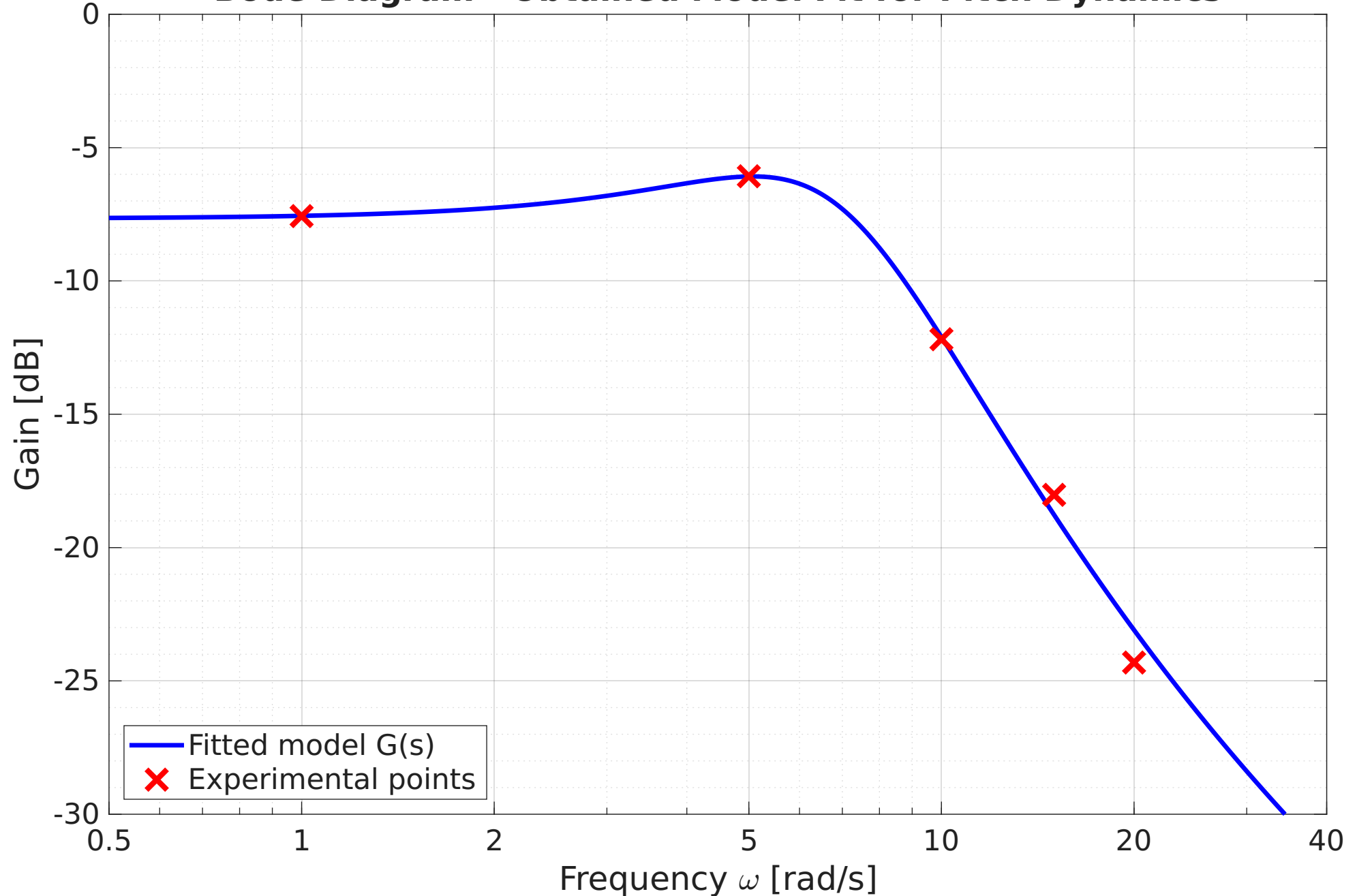
Bode Diagram - Obtained Model Fit for Pitch Dynamics
