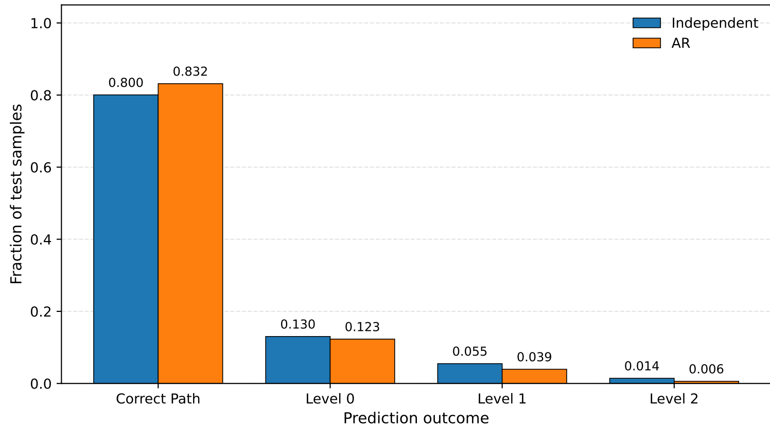
Hierarchical Prediction Outcomes
