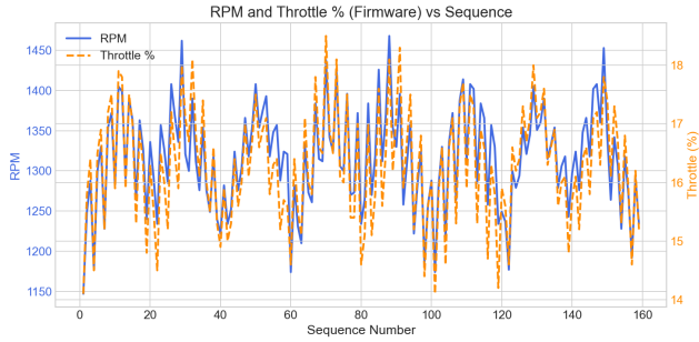
Fig. 7: Rpm Throttle
