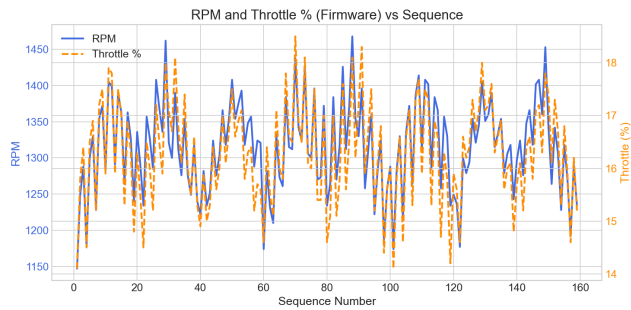
Fig. 7: Rpm Throttle
