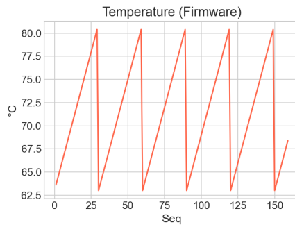
Fig. 5: Temperature
