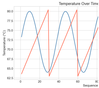
Fig. 5: Temperature
