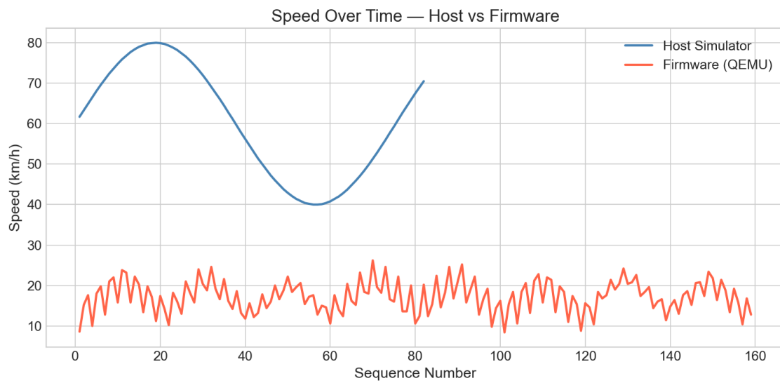
Figure 6: Speed Comparison
