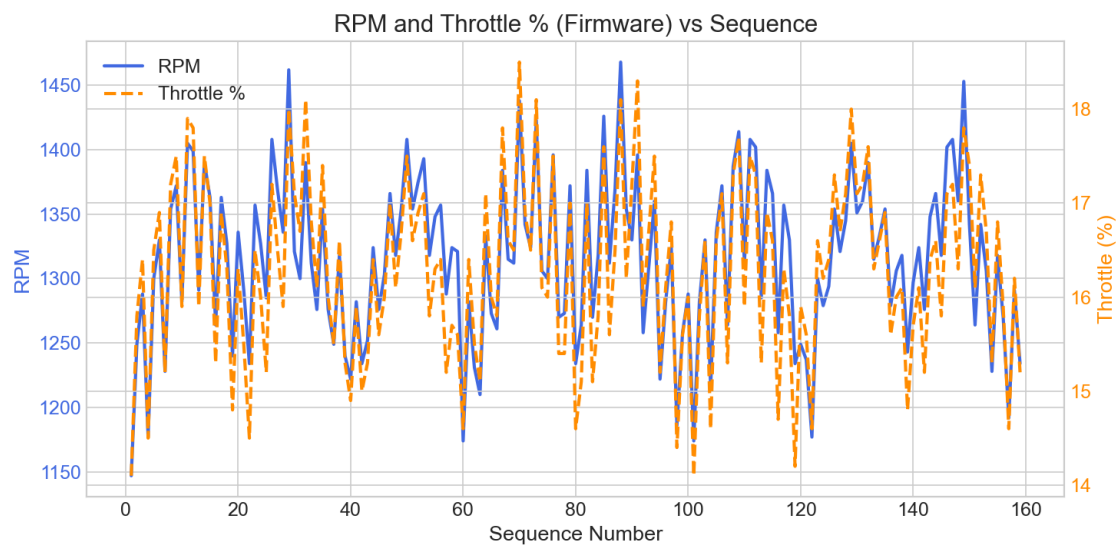
Figure 7: Rpm Throttle
