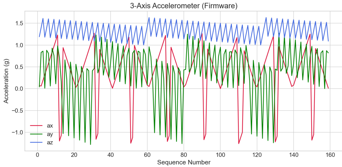
Figure 9: Firmware Acceleration 3Axis
