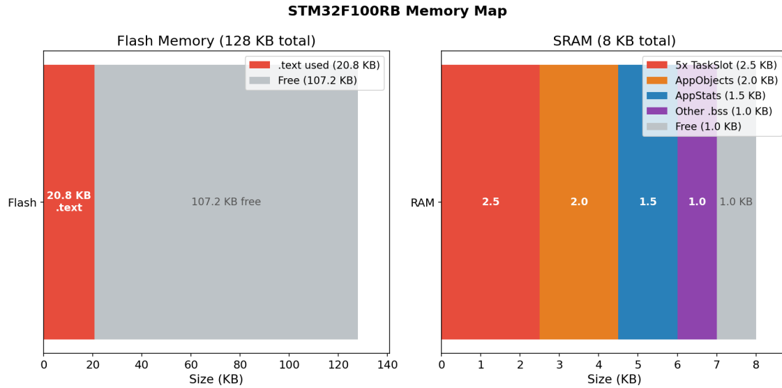
Figure 13: Memory Map
