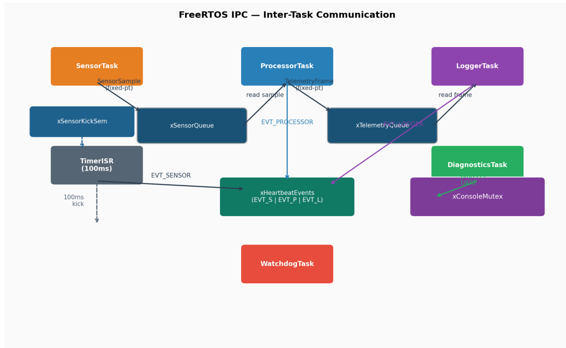
Figure 3: Ipc Diagram
