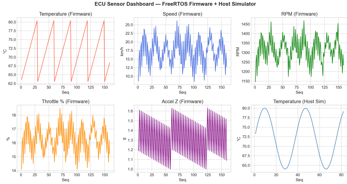
Figure 8: Sensor Dashboard
