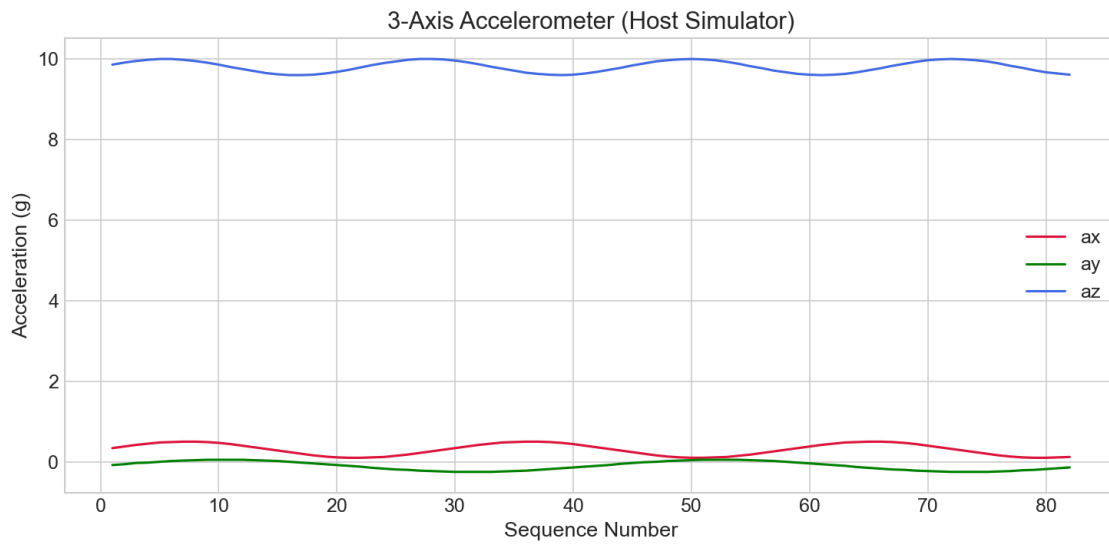
Figure 10: Host Acceleration 3Axis
