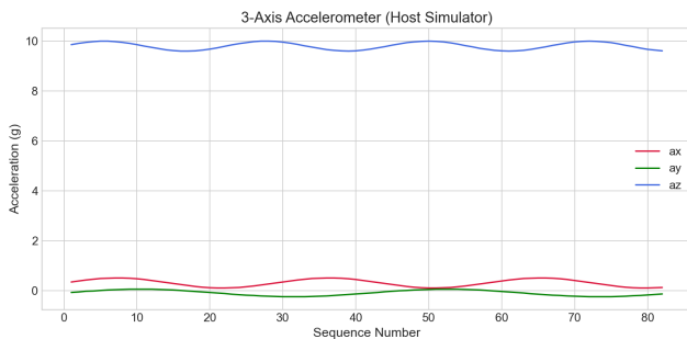
Fig. 10: Host Acceleration 3Axis
