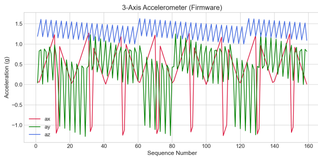
Fig. 9: Firmware Acceleration 3Axis
