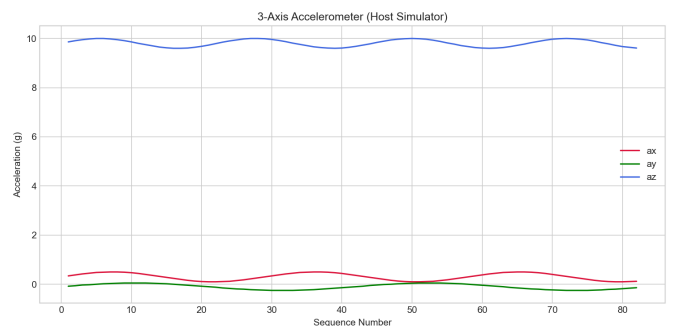
Fig. 10. Host Acceleration 3Axis
