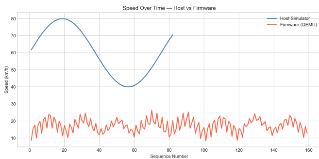
Fig. 6. Speed Comparison
