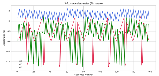
Fig. 9. Firmware Acceleration 3Axis
