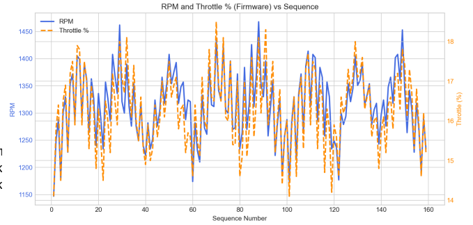
Fig. 7. Rpm Throttle
