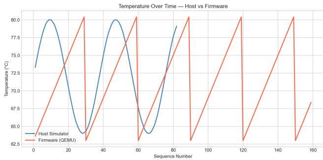
Fig. 5. Temperature Comparison
