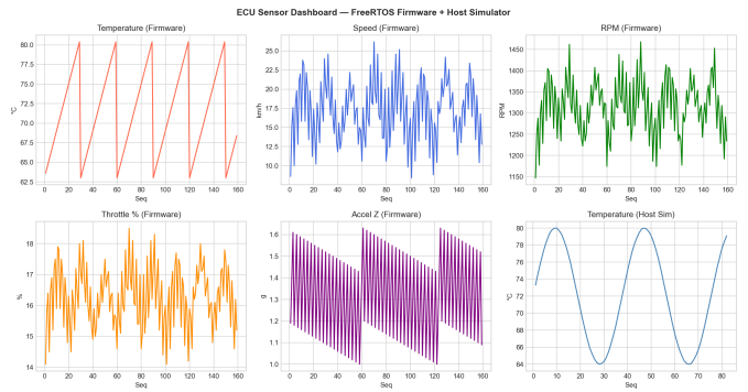
Fig. 8. Sensor Dashboard
