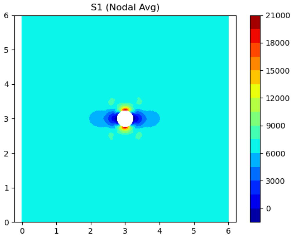
Figure 18: CQ8/CQ7 Open Hole Plate Results
