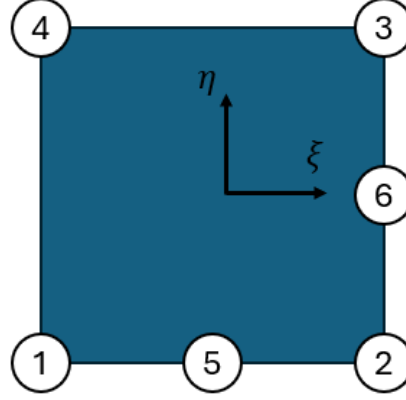
Figure 13: CQUAD6 Element
