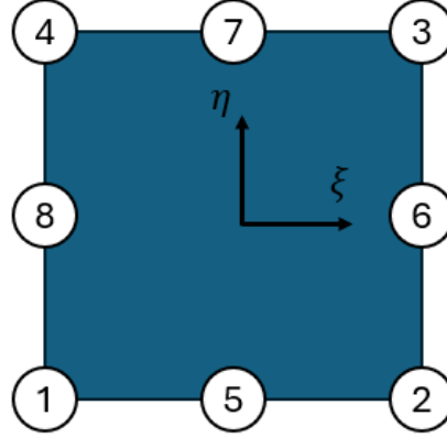
Figure 11: CQUAD8 Element
