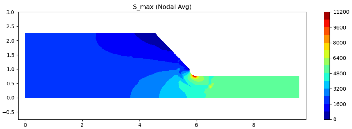
Figure 26: CQ8_16 Max Principal Stress (psi)
