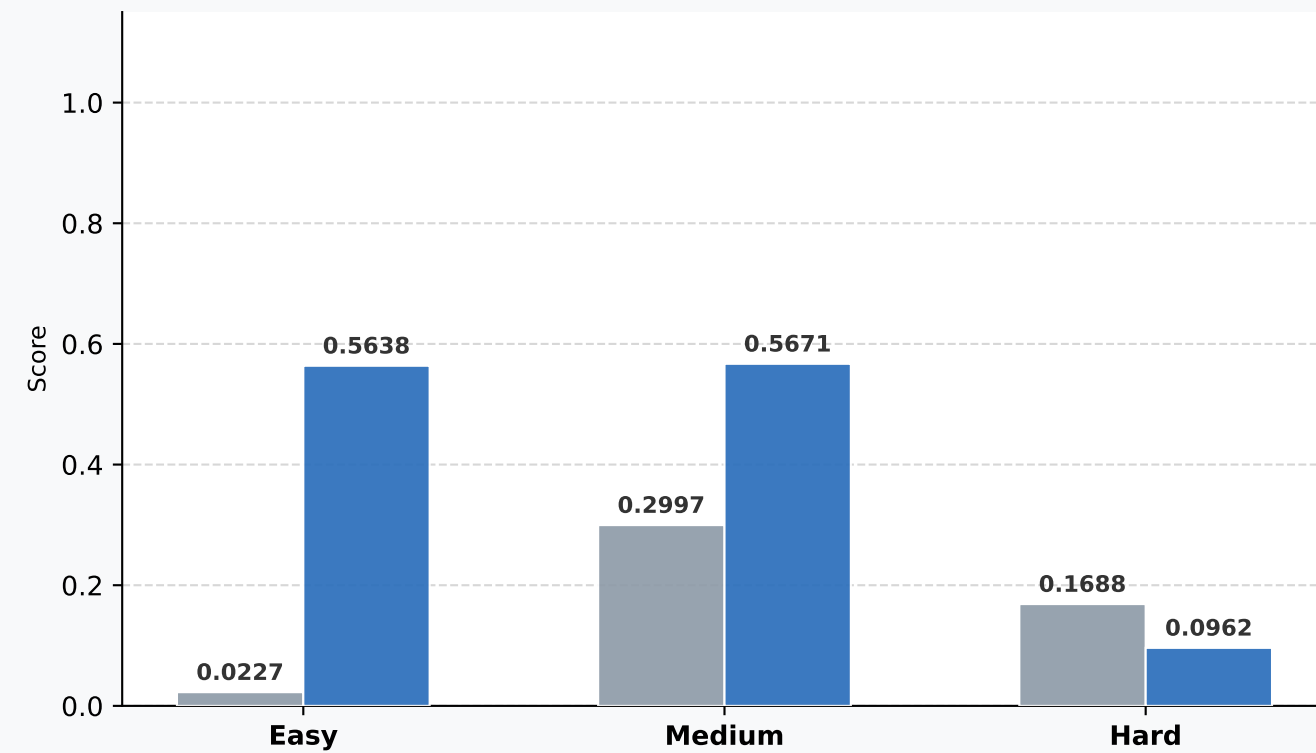
Context Recall
