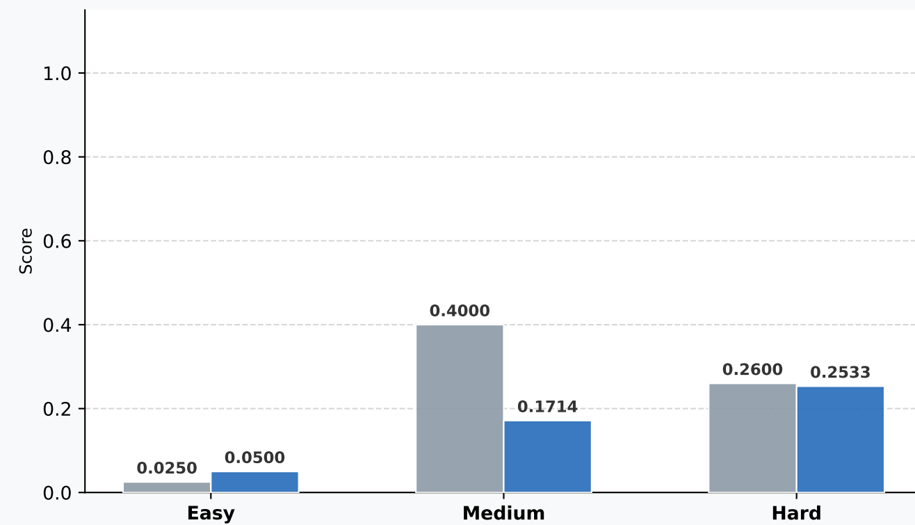
Context Recall
