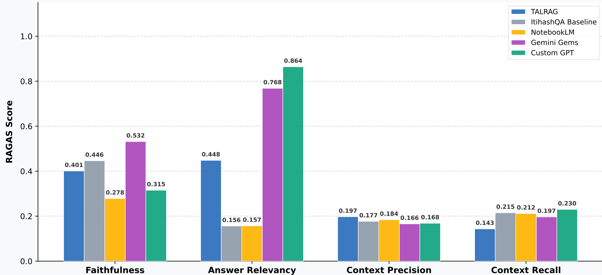
Overall RAGAS Performance — 5 System Comparison
